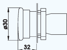
RP2-BS44+RP2-BZ10=RCP2-BS44
