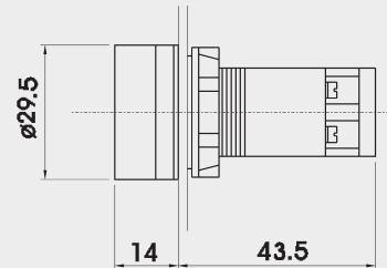
RCP7-IVL-7●
