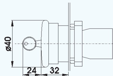
RP2-BS14+RP2-BZ10=RCP2-BS14
