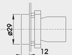
RP2-BA+RP2-BZ10=RCP2-BA RP2-BA334+RP2-BZ10=RCP2-BA334
